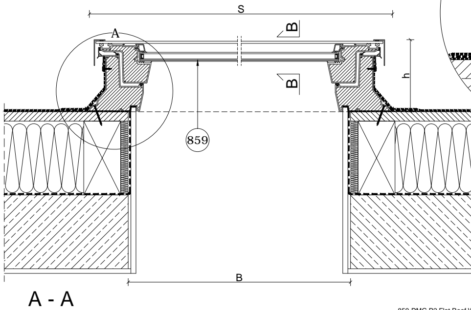
859-DMG P2 Flat Roof Window, opened manually
